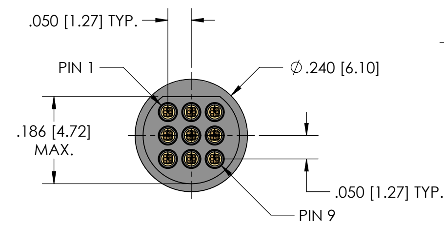
9 POSITION PLUG
