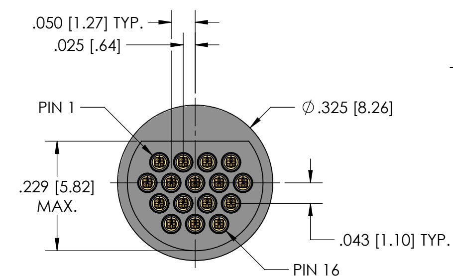
16 POSITION PLUG
