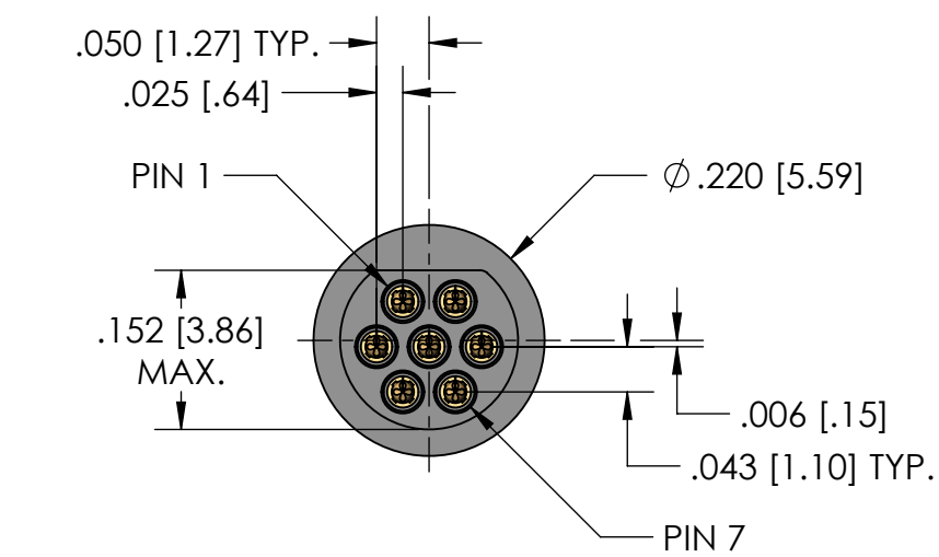
7 POSITION PLUG
