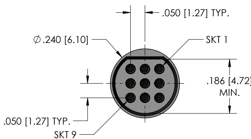
9 POSITION RECEPTACLE
