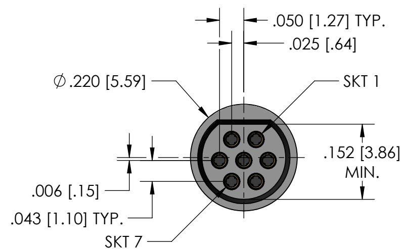
7 POSITION RECEPTACLE
