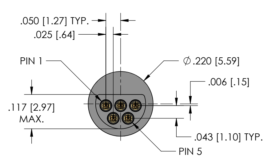
5 POSITION PLUG
