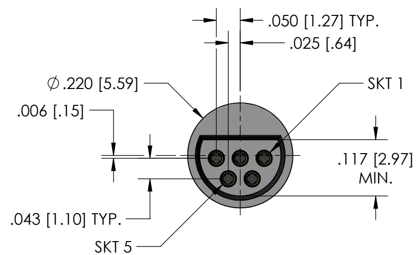
5 POSITION RECEPTACLE
