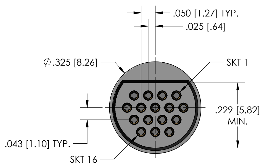
16 POSITION RECEPTACLE
